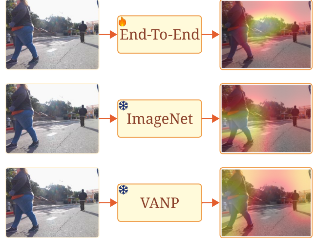
Fig. 1: Comparison of Activation Maps Learned by End-to-End, ImageNet, and VANP. VANP can extract multiple regions of interest for navigation without downstream navigation supervision compared to single salient regions by End-to-End and ImageNet pre-trained models.
